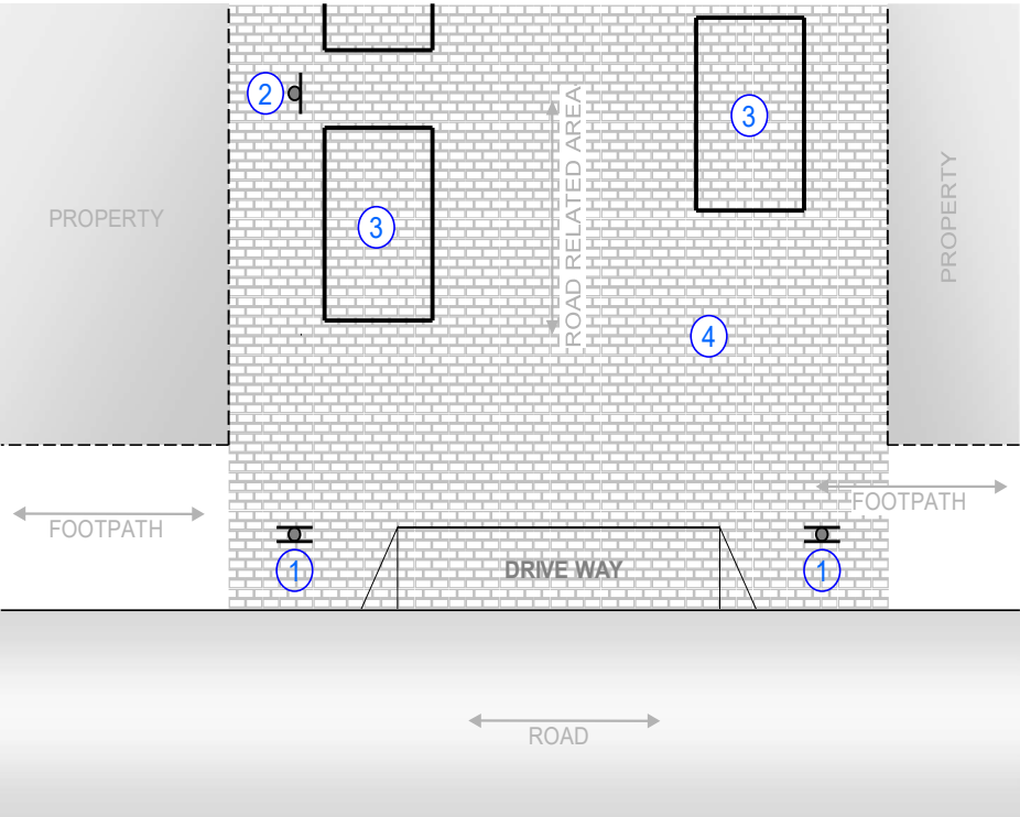
Category 1 shared zone Indicative layout and treatments
